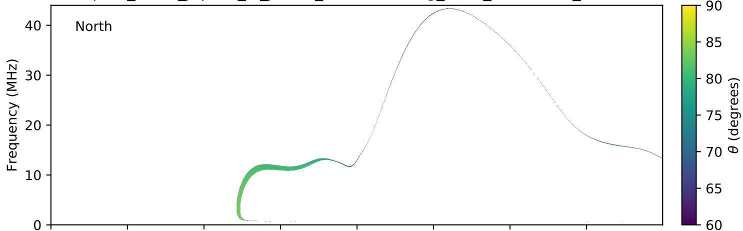
expres_earth_jupiter_io_jrm09_lossc-wid1deg_3kev_20161212_v01.cdf
