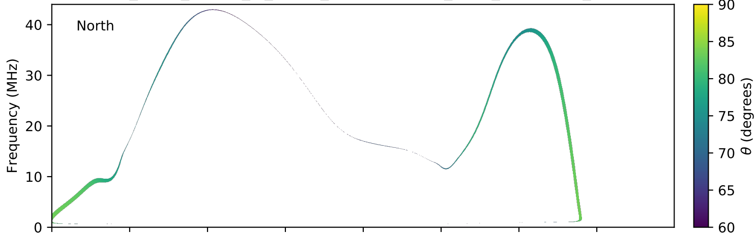
expres_earth_jupiter_io_jrm09_lossc-wid1deg_3kev_20161207_v01.cdf
