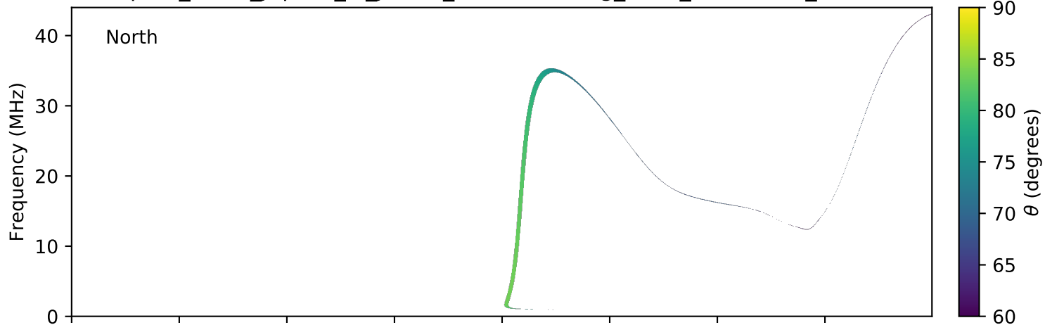
expres_earth_jupiter_io_jrm09_lossc-wid1deg_3kev_20161203_v01.cdf
