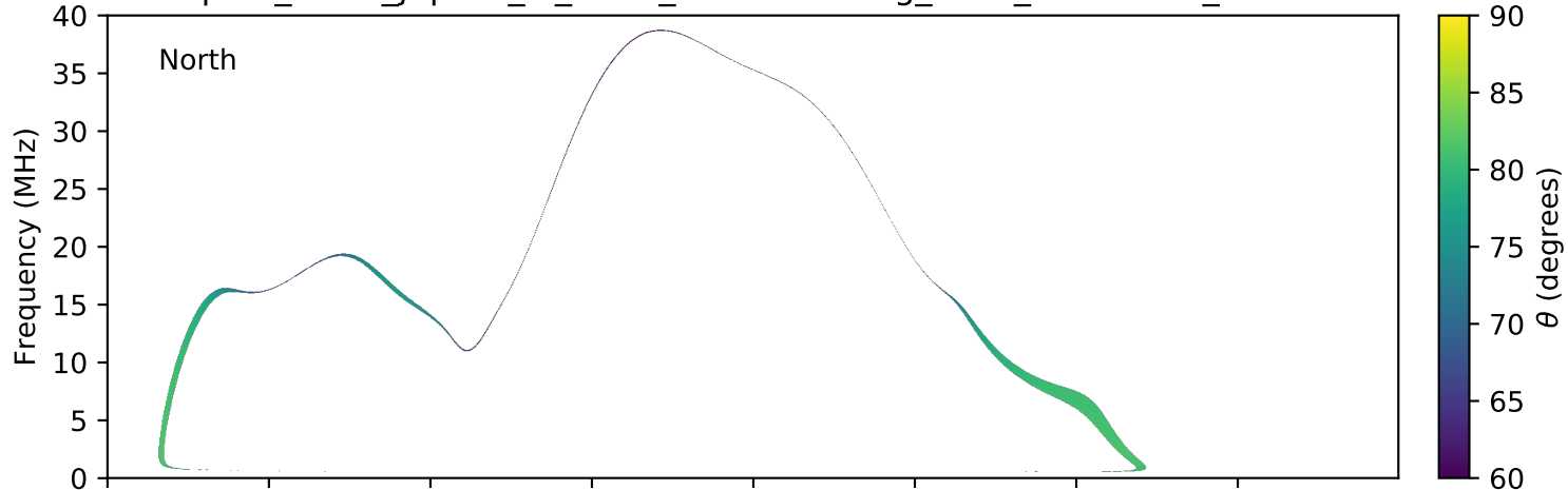
expres_earth_jupiter_io_isaac_lossc-wid1deg_5kev_20161230_v01.cdf
