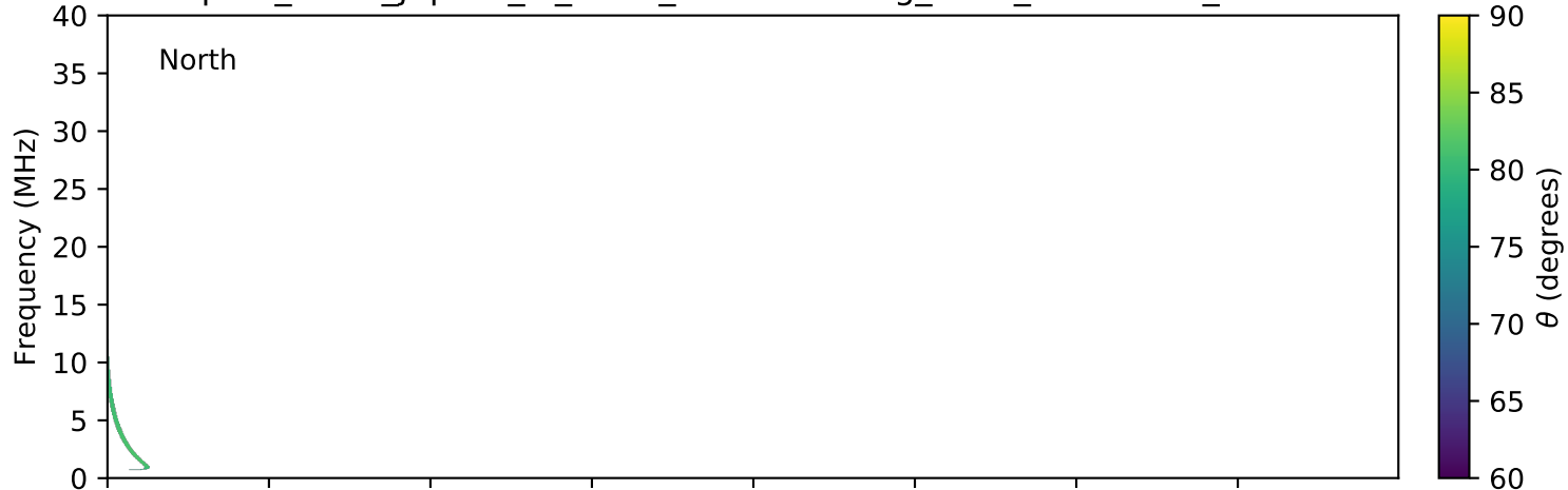
expres_earth_jupiter_io_isaac_lossc-wid1deg_5kev_20161229_v01.cdf
