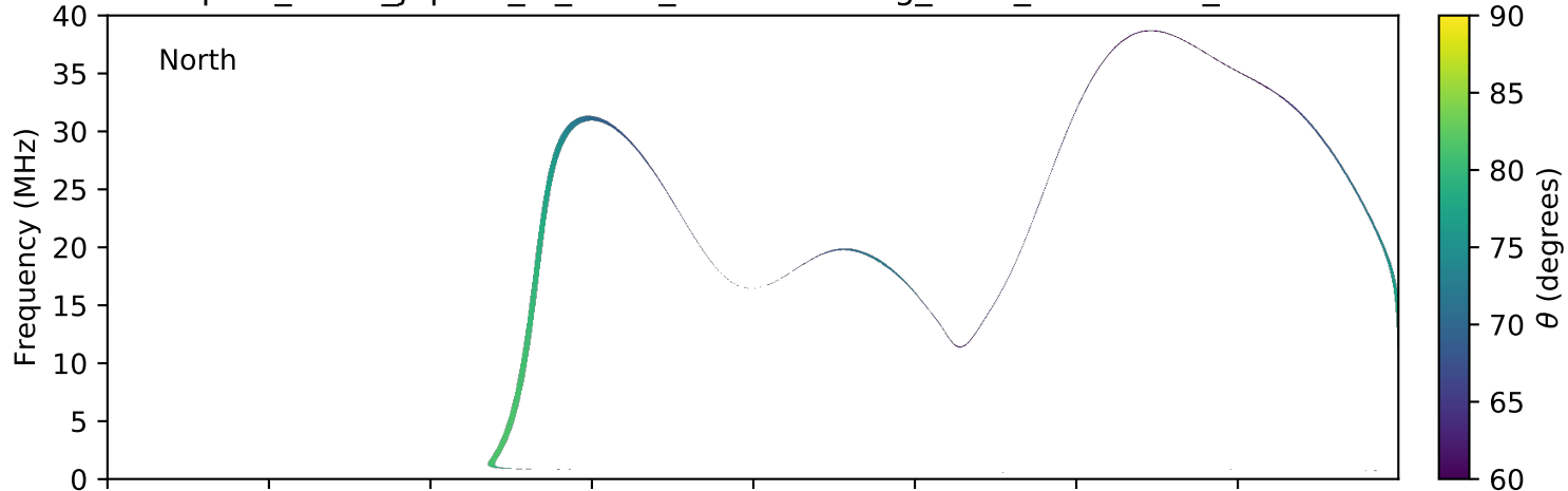
expres_earth_jupiter_io_isaac_lossc-wid1deg_5kev_20161228_v01.cdf
