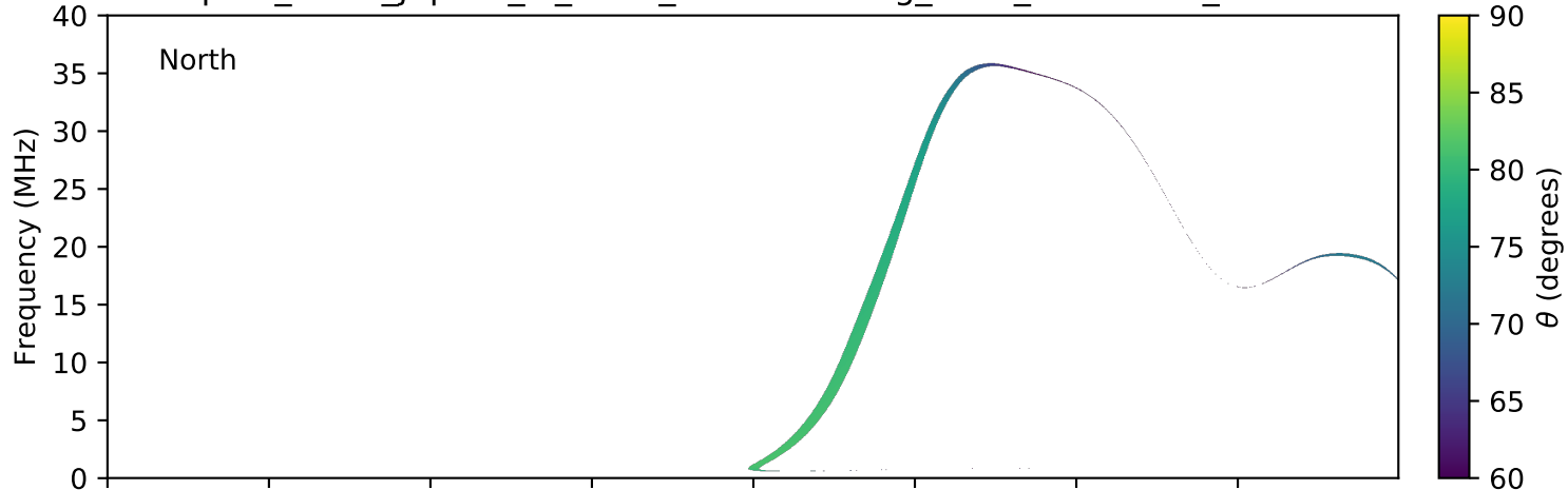
expres_earth_jupiter_io_isaac_lossc-wid1deg_5kev_20161226_v01.cdf
