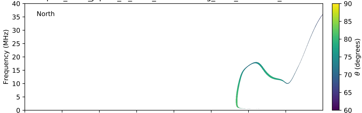
expres_earth_jupiter_io_isaac_lossc-wid1deg_5kev_20161224_v01.cdf
