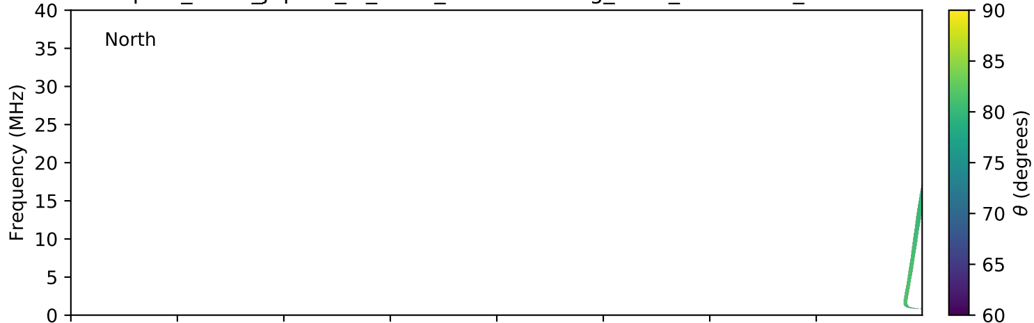
expres_earth_jupiter_io_isaac_lossc-wid1deg_5kev_20161222_v01.cdf
