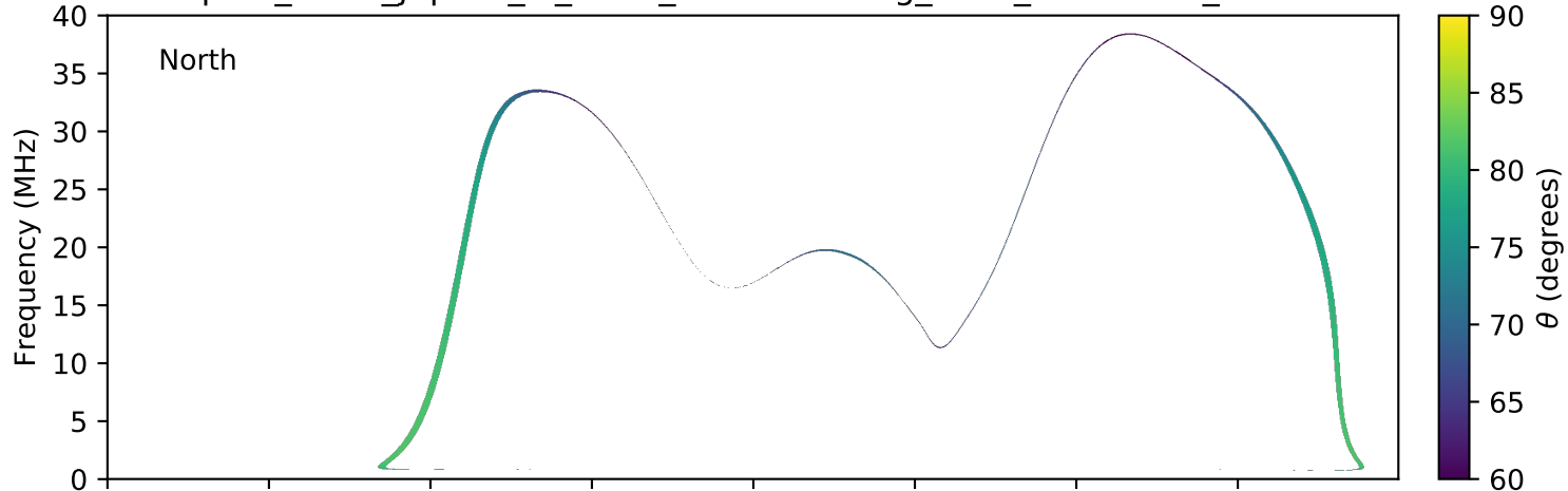
expres_earth_jupiter_io_isaac_lossc-wid1deg_5kev_20161221_v01.cdf
