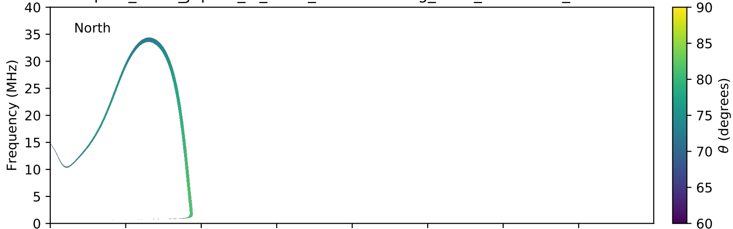
expres_earth_jupiter_io_isaac_lossc-wid1deg_5kev_20161220_v01.cdf
