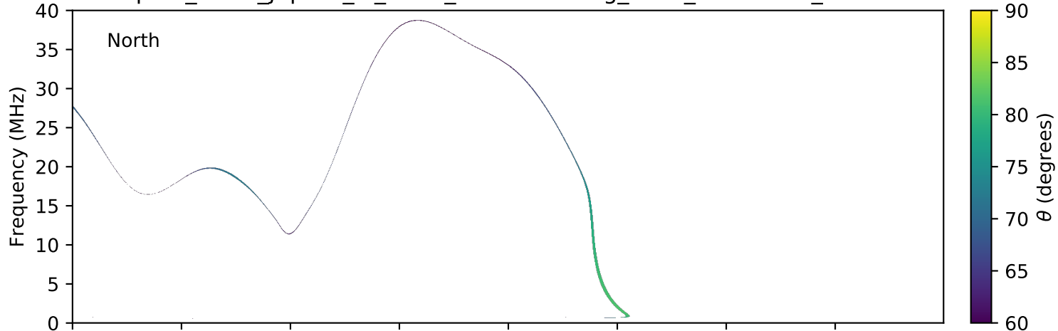
expres_earth_jupiter_io_isaac_lossc-wid1deg_5kev_20161216_v01.cdf
