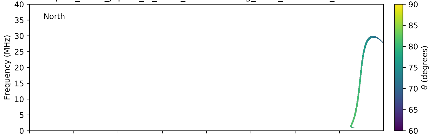
expres_earth_jupiter_io_isaac_lossc-wid1deg_5kev_20161215_v01.cdf
