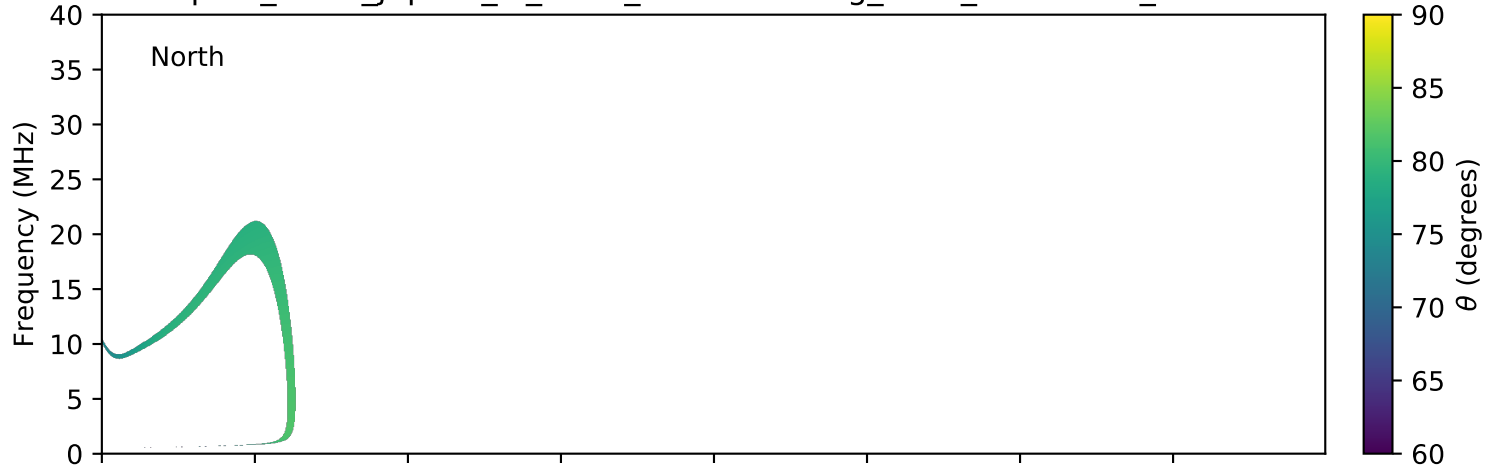
expres_earth_jupiter_io_isaac_lossc-wid1deg_5kev_20161213_v01.cdf
