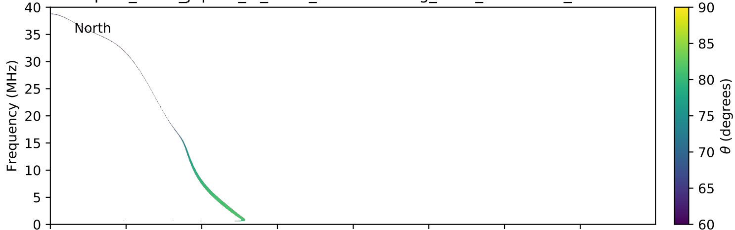
expres_earth_jupiter_io_isaac_lossc-wid1deg_5kev_20161211_v01.cdf
