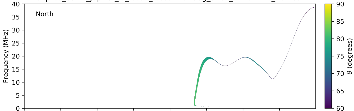
expres_earth_jupiter_io_isaac_lossc-wid1deg_5kev_20161210_v01.cdf
