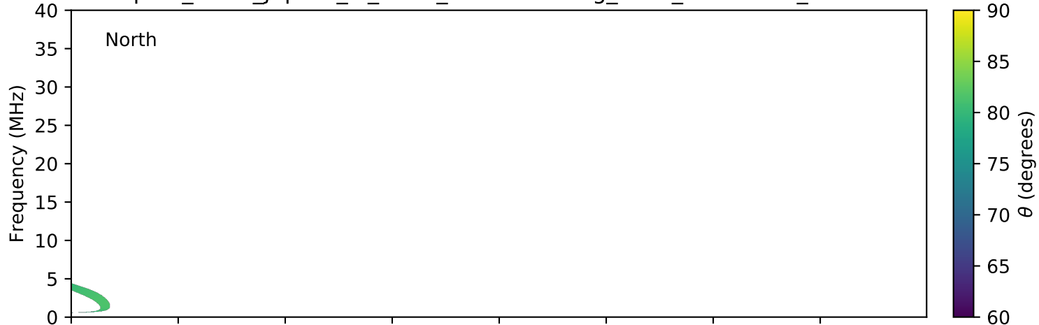
expres_earth_jupiter_io_isaac_lossc-wid1deg_5kev_20161206_v01.cdf
