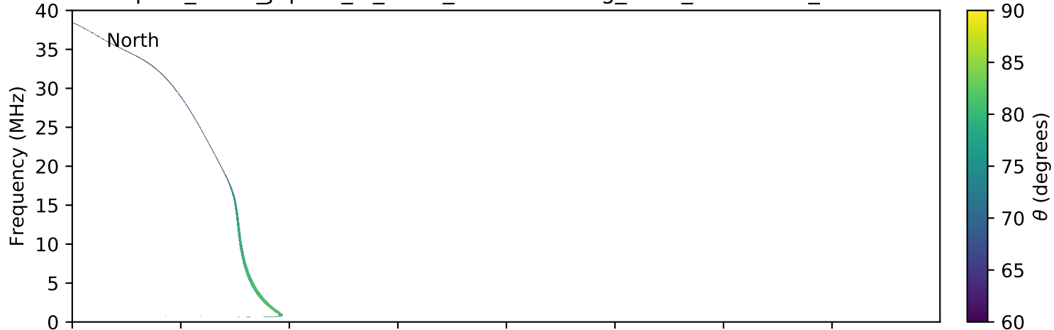
expres_earth_jupiter_io_isaac_lossc-wid1deg_5kev_20161204_v01.cdf
