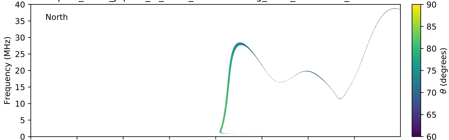
expres_earth_jupiter_io_isaac_lossc-wid1deg_5kev_20161203_v01.cdf
