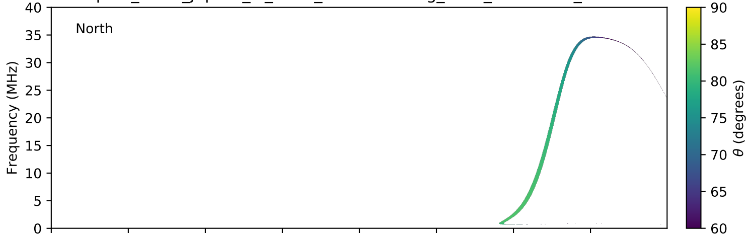
expres_earth_jupiter_io_isaac_lossc-wid1deg_5kev_20161201_v01.cdf
