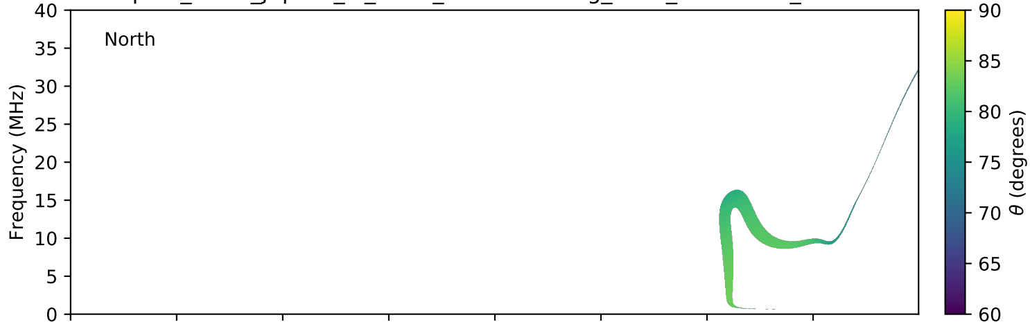
expres_earth_jupiter_io_isaac_lossc-wid1deg_3kev_20161231_v01.cdf
