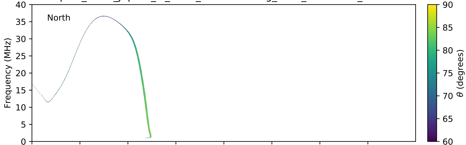
expres_earth_jupiter_io_isaac_lossc-wid1deg_3kev_20161227_v01.cdf
