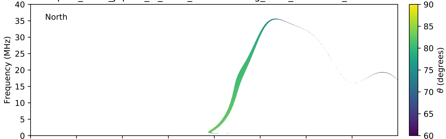
expres_earth_jupiter_io_isaac_lossc-wid1deg_3kev_20161226_v01.cdf
