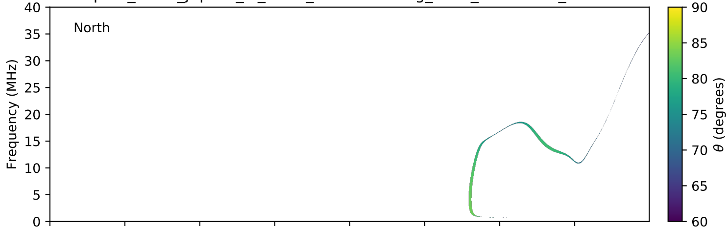
expres_earth_jupiter_io_isaac_lossc-wid1deg_3kev_20161224_v01.cdf
