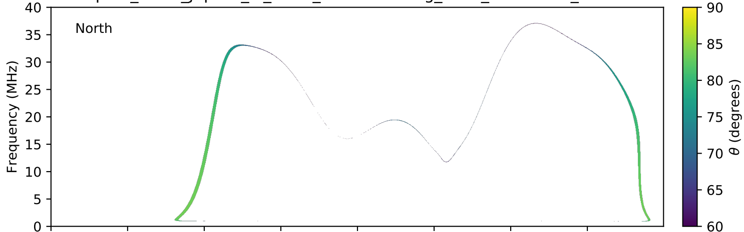
expres_earth_jupiter_io_isaac_lossc-wid1deg_3kev_20161221_v01.cdf
