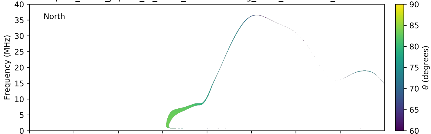
expres_earth_jupiter_io_isaac_lossc-wid1deg_3kev_20161219_v01.cdf
