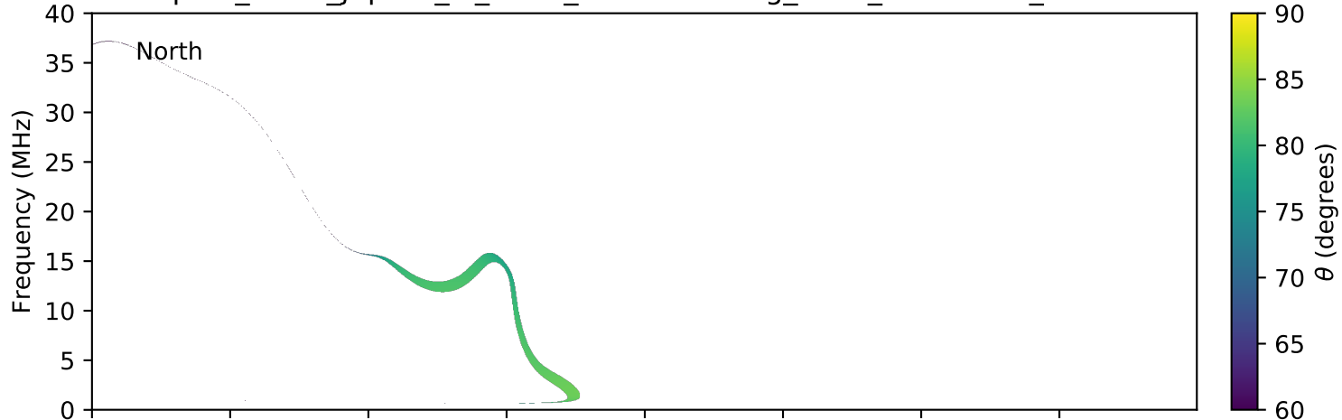
expres_earth_jupiter_io_isaac_lossc-wid1deg_3kev_20161218_v01.cdf
