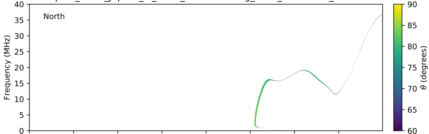
expres_earth_jupiter_io_isaac_lossc-wid1deg_3kev_20161217_v01.cdf
