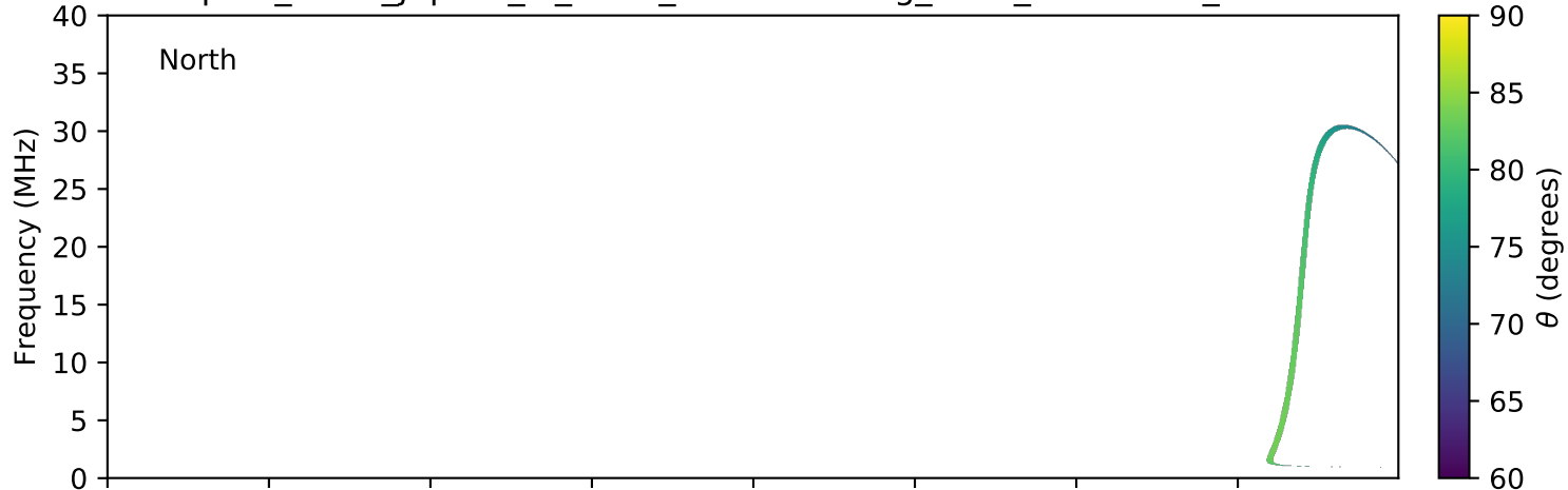
expres_earth_jupiter_io_isaac_lossc-wid1deg_3kev_20161215_v01.cdf
