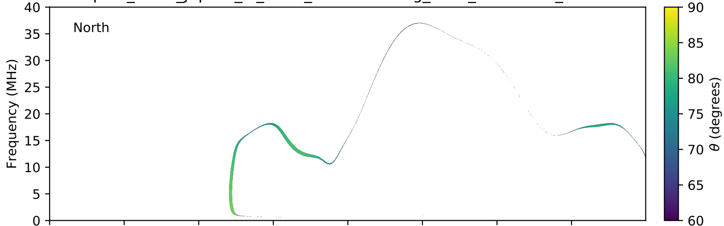
expres_earth_jupiter_io_isaac_lossc-wid1deg_3kev_20161212_v01.cdf
