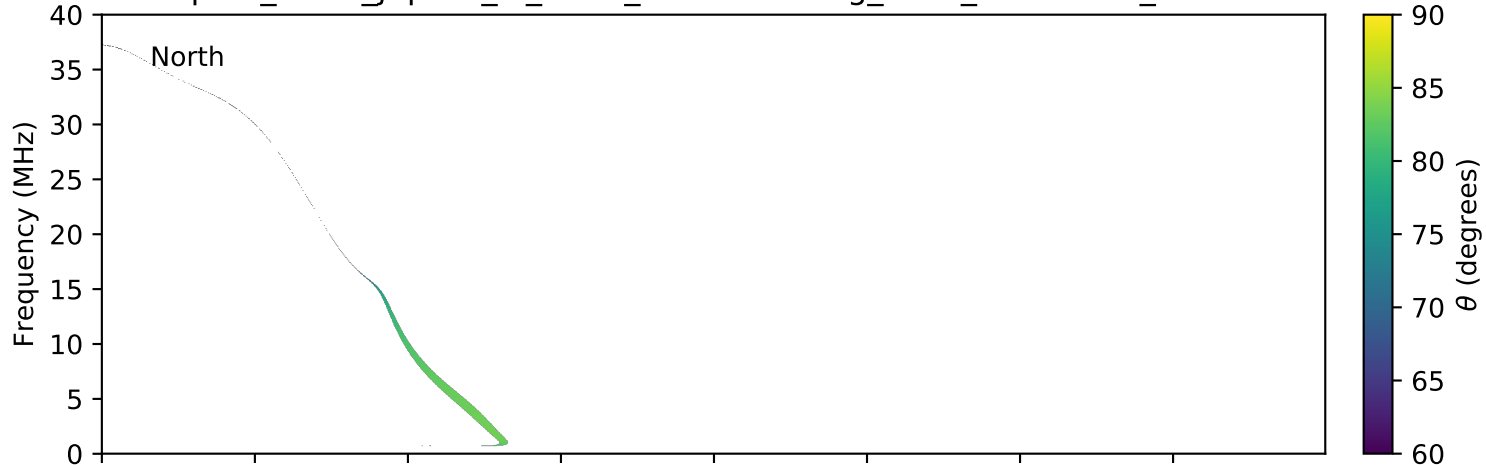
expres_earth_jupiter_io_isaac_lossc-wid1deg_3kev_20161211_v01.cdf
