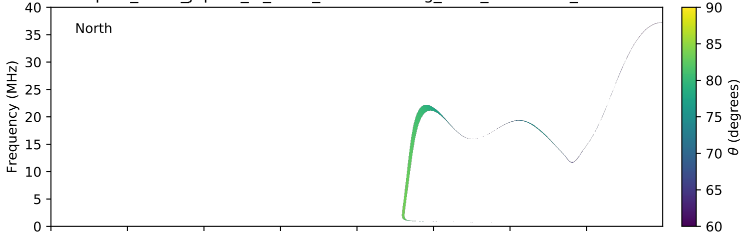
expres_earth_jupiter_io_isaac_lossc-wid1deg_3kev_20161210_v01.cdf
