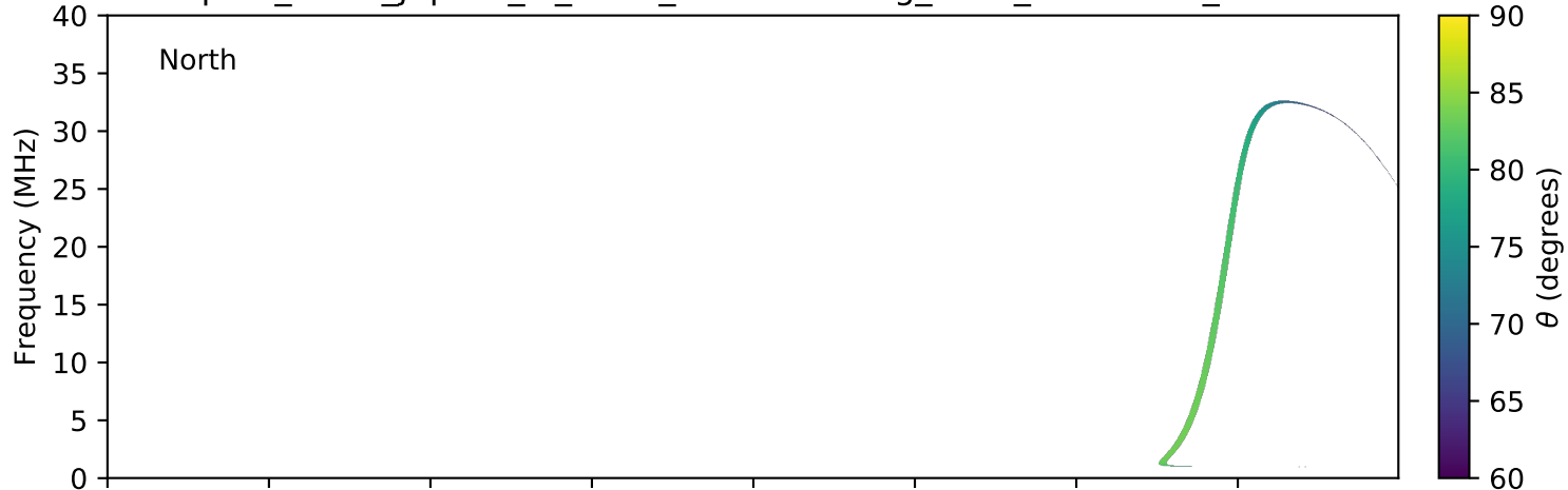
expres_earth_jupiter_io_isaac_lossc-wid1deg_3kev_20161208_v01.cdf
