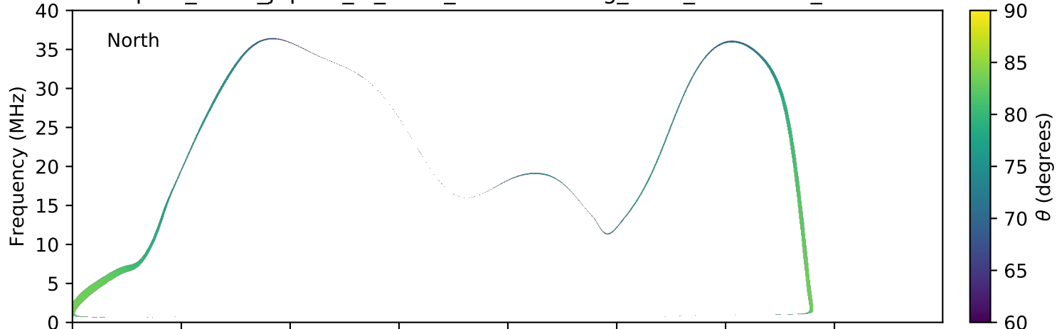
expres_earth_jupiter_io_isaac_lossc-wid1deg_3kev_20161207_v01.cdf
