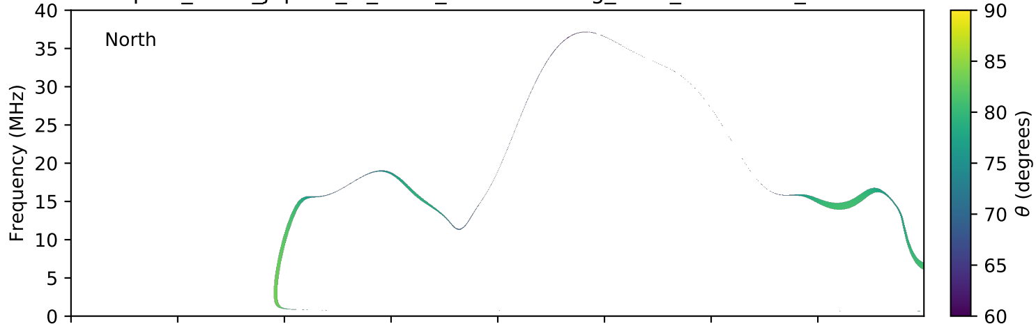
expres_earth_jupiter_io_isaac_lossc-wid1deg_3kev_20161205_v01.cdf
