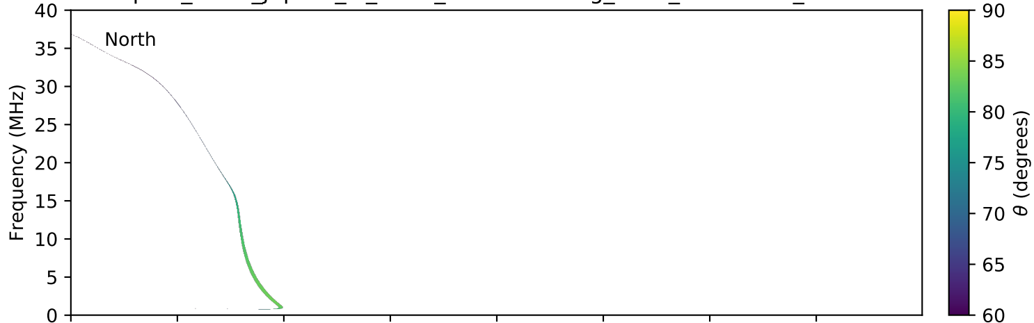
expres_earth_jupiter_io_isaac_lossc-wid1deg_3kev_20161204_v01.cdf
