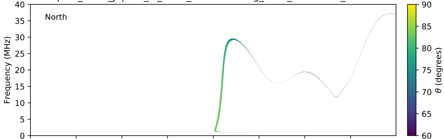
expres_earth_jupiter_io_isaac_lossc-wid1deg_3kev_20161203_v01.cdf
