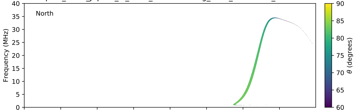
expres_earth_jupiter_io_isaac_lossc-wid1deg_3kev_20161201_v01.cdf
