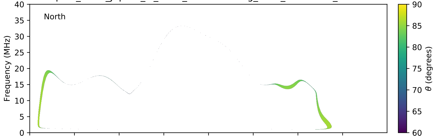
expres_earth_jupiter_io_isaac_lossc-wid1deg_1kev_20161230_v01.cdf
