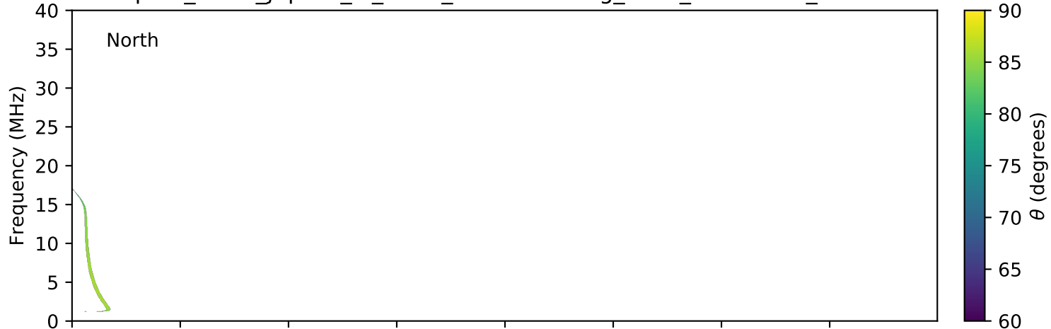
expres_earth_jupiter_io_isaac_lossc-wid1deg_1kev_20161229_v01.cdf
