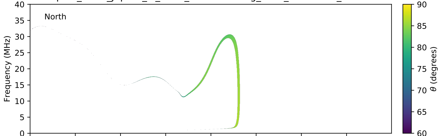
expres_earth_jupiter_io_isaac_lossc-wid1deg_1kev_20161225_v01.cdf
