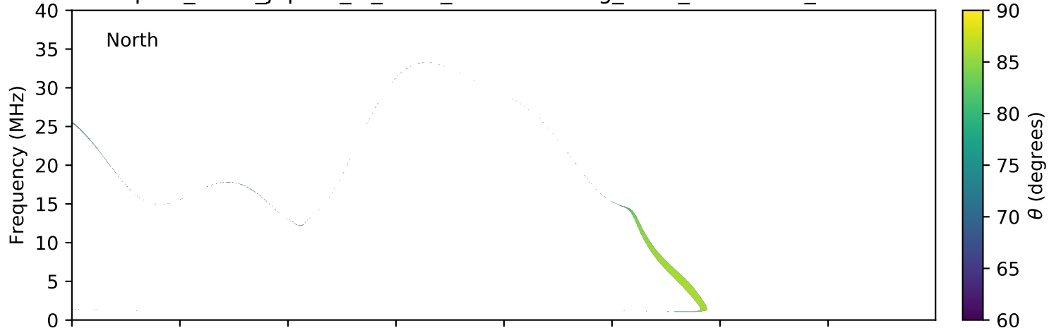
expres_earth_jupiter_io_isaac_lossc-wid1deg_1kev_20161223_v01.cdf
