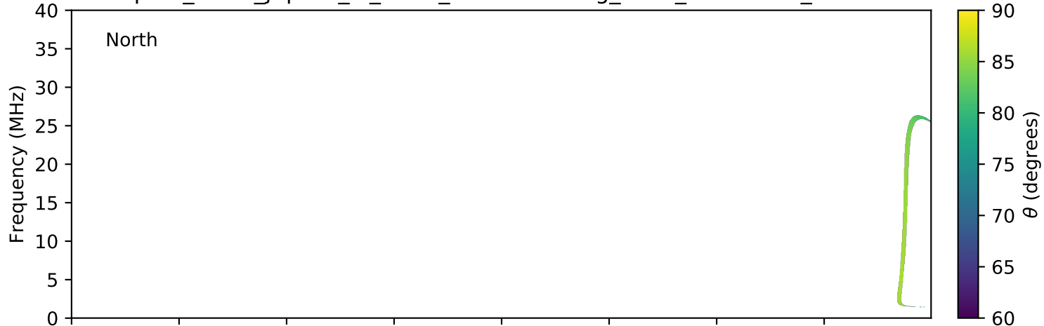
expres_earth_jupiter_io_isaac_lossc-wid1deg_1kev_20161222_v01.cdf
