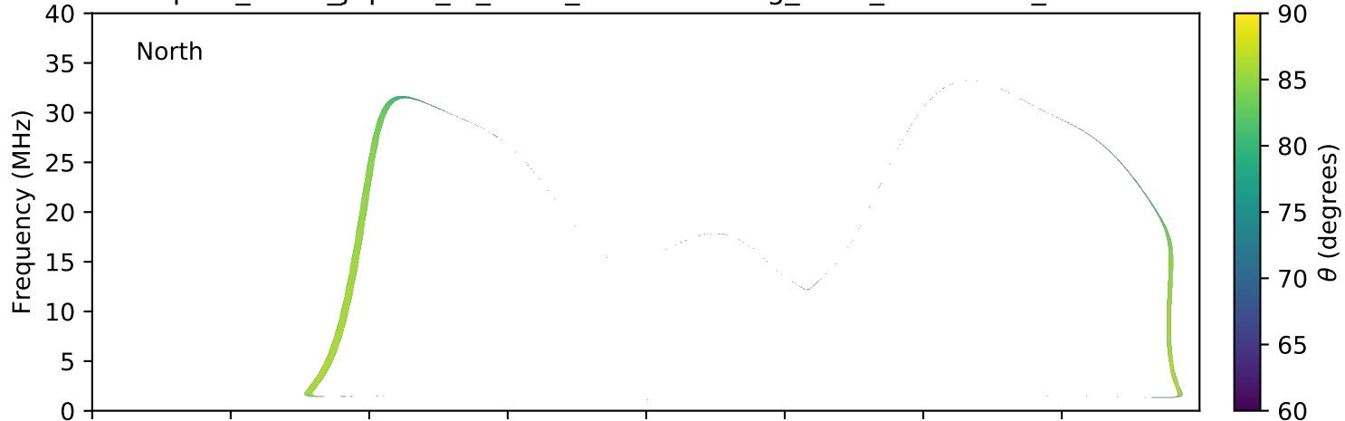
expres_earth_jupiter_io_isaac_lossc-wid1deg_1kev_20161221_v01.cdf
