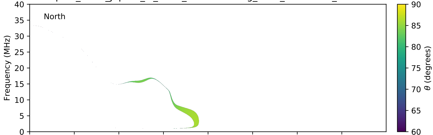
expres_earth_jupiter_io_isaac_lossc-wid1deg_1kev_20161218_v01.cdf
