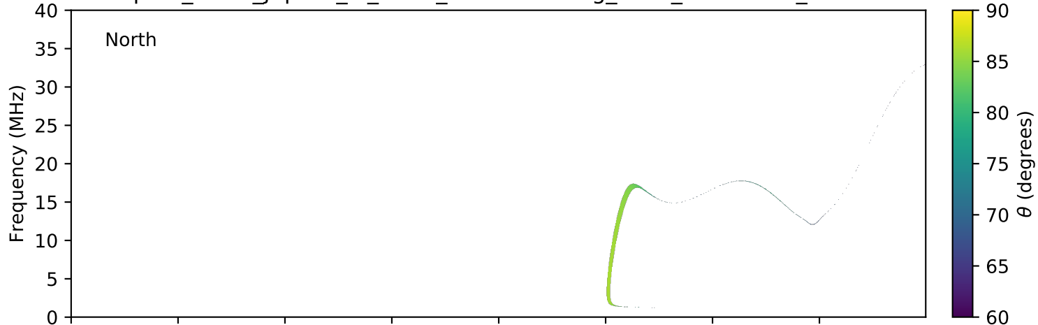
expres_earth_jupiter_io_isaac_lossc-wid1deg_1kev_20161217_v01.cdf
