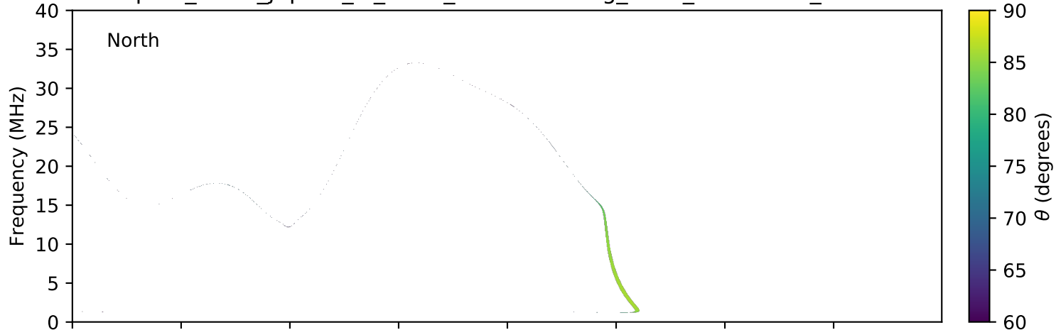
expres_earth_jupiter_io_isaac_lossc-wid1deg_1kev_20161216_v01.cdf
