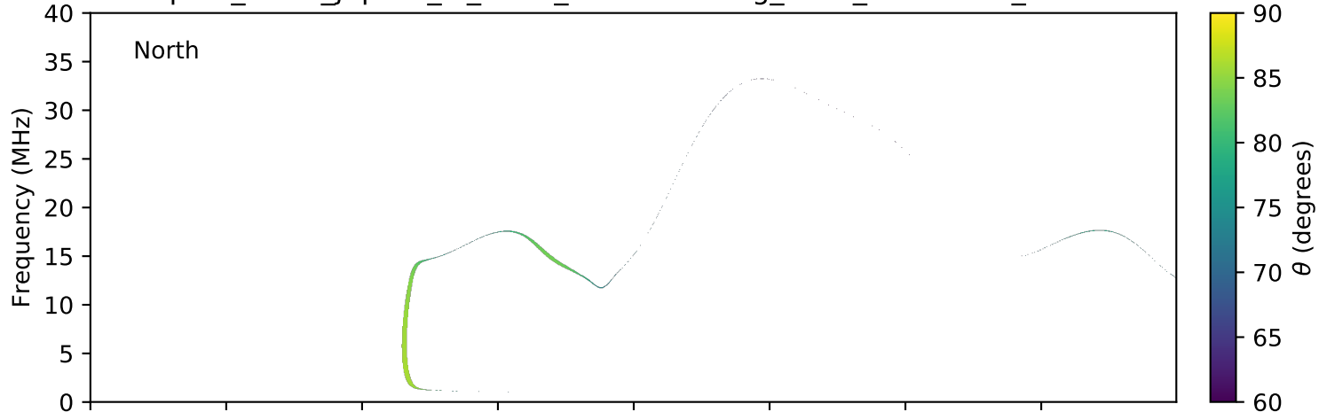
expres_earth_jupiter_io_isaac_lossc-wid1deg_1kev_20161212_v01.cdf
