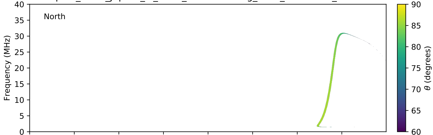
expres_earth_jupiter_io_isaac_lossc-wid1deg_1kev_20161208_v01.cdf
