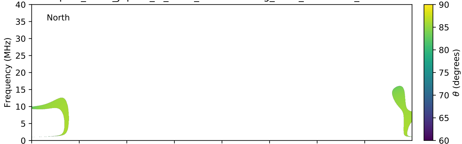
expres_earth_jupiter_io_isaac_lossc-wid1deg_1kev_20161206_v01.cdf
